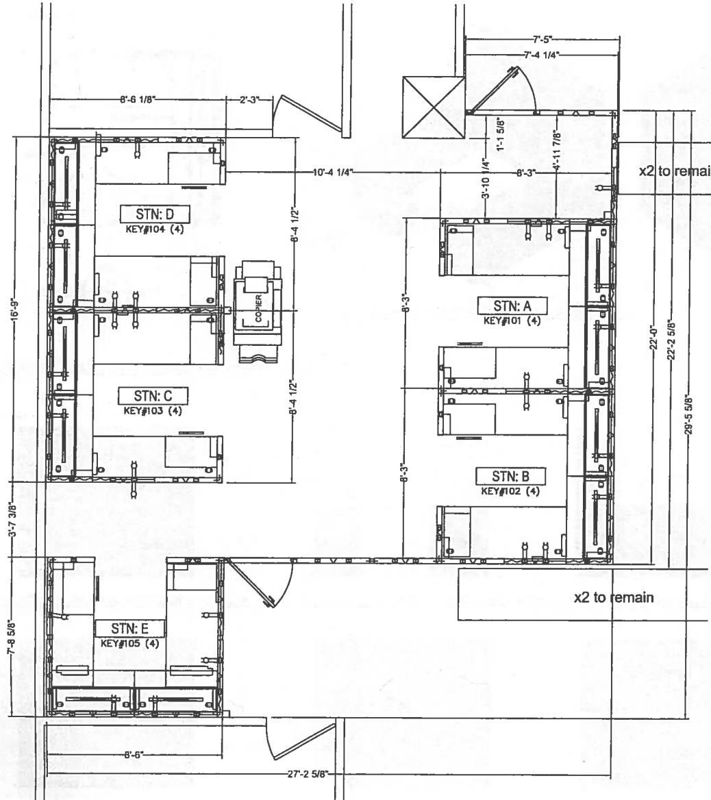
1 OVERALL FLOOR PLAN SCALE: 1/2" = 1'-0"
